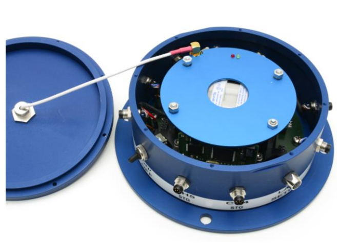
Encoder inside
