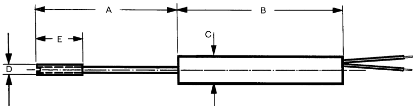
Type WLH economic, compact sensor
